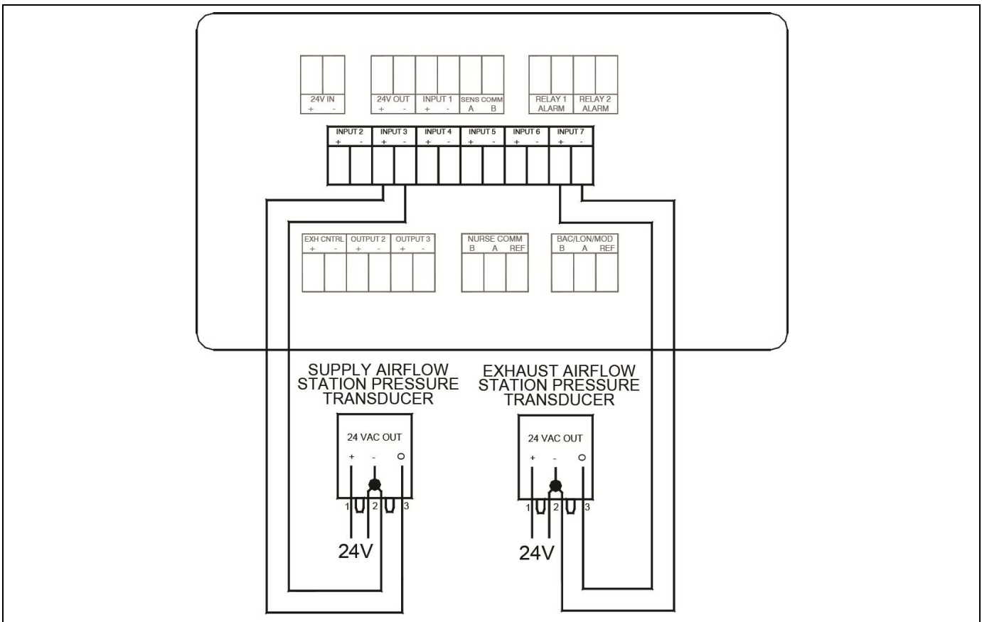
Figure 11. Optional Supply / Exhaust Pressure-Based Flow Station Wiring to Model RPM10 / RPM20
