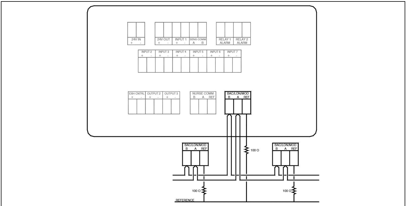
Figure 21. Optional Modbus and BACnet MS/TP Communications Wiring to Model RPM10 / RPM20
