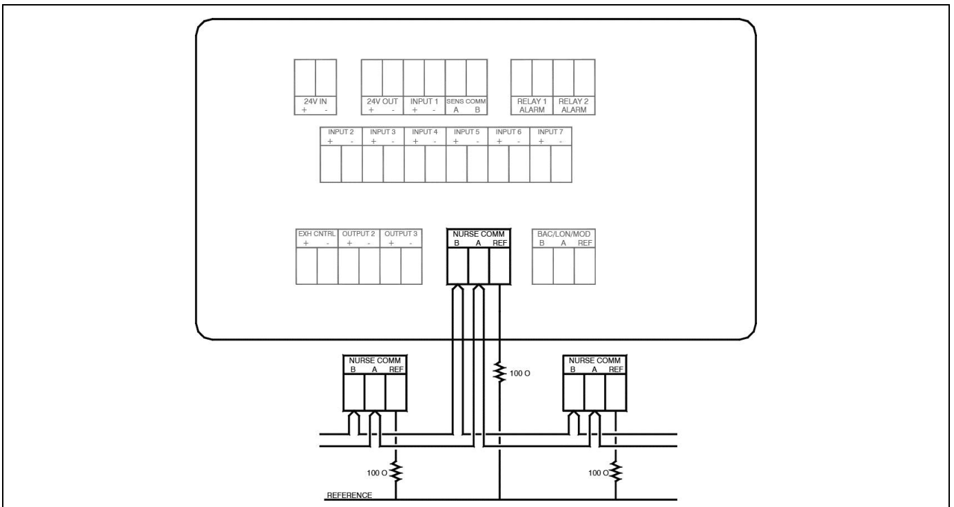
Figure 20. Optional Nurses Station Communications Wiring to Model RPM10 / RPM20
