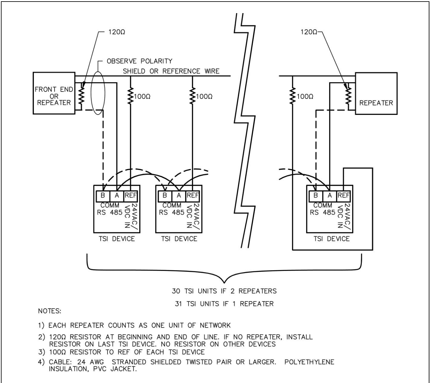
Figure 23. Proper Communication Wiring Diagram
