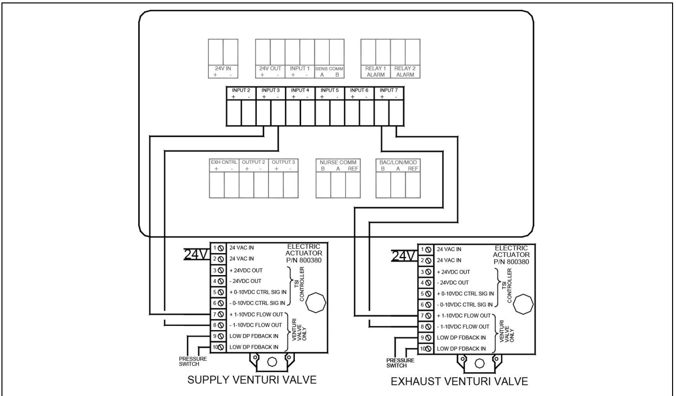
Figure 13. Optional Supply / Exhaust Venturi Valve Wiring to Model RPM10 / RPM20
